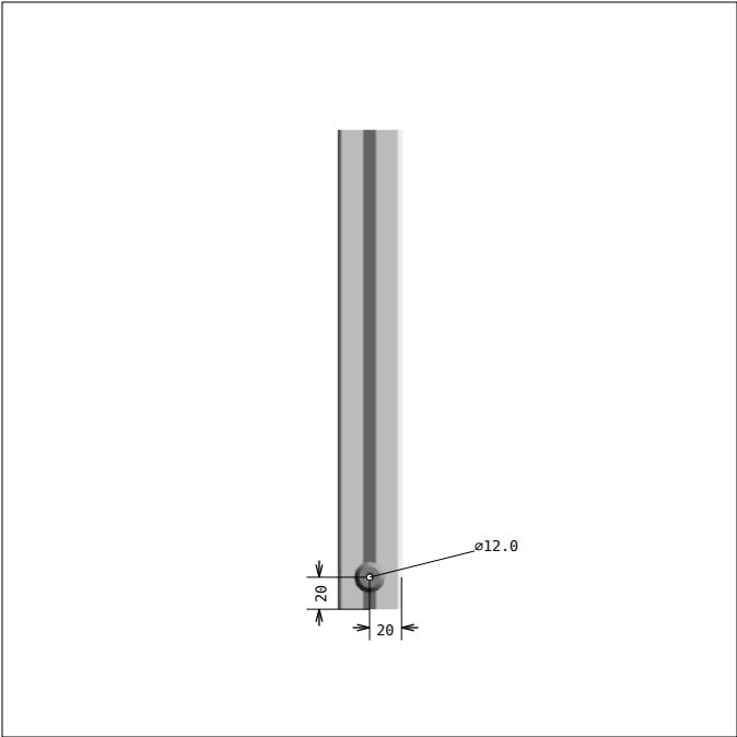
DRAWING 1, Pos 1 SIDE 1, bar length: 300.0 mm
